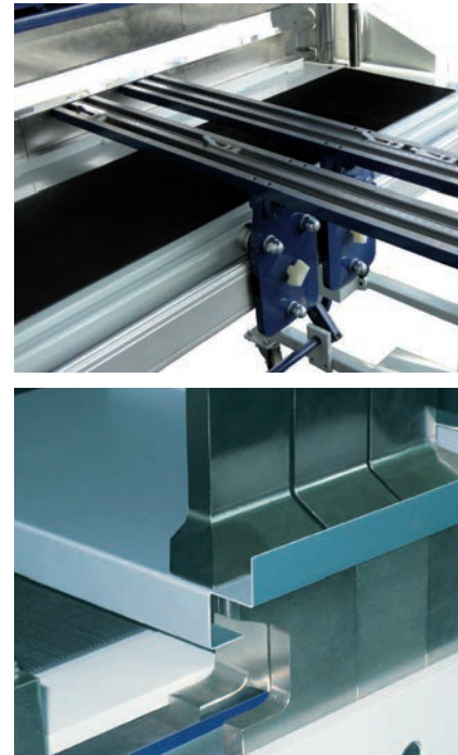
Variable stop bars enable precision (image above). Open new possibilities: segmented tools on all three beams (image below)
